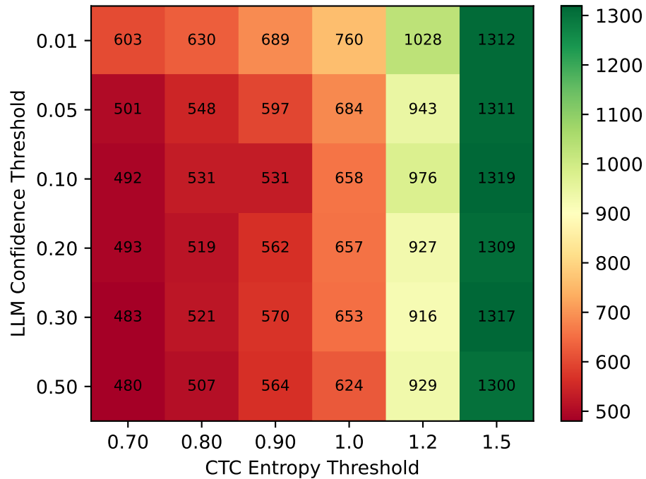
RTF x
