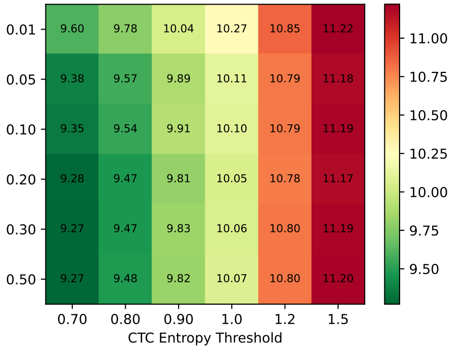
WER (%)
